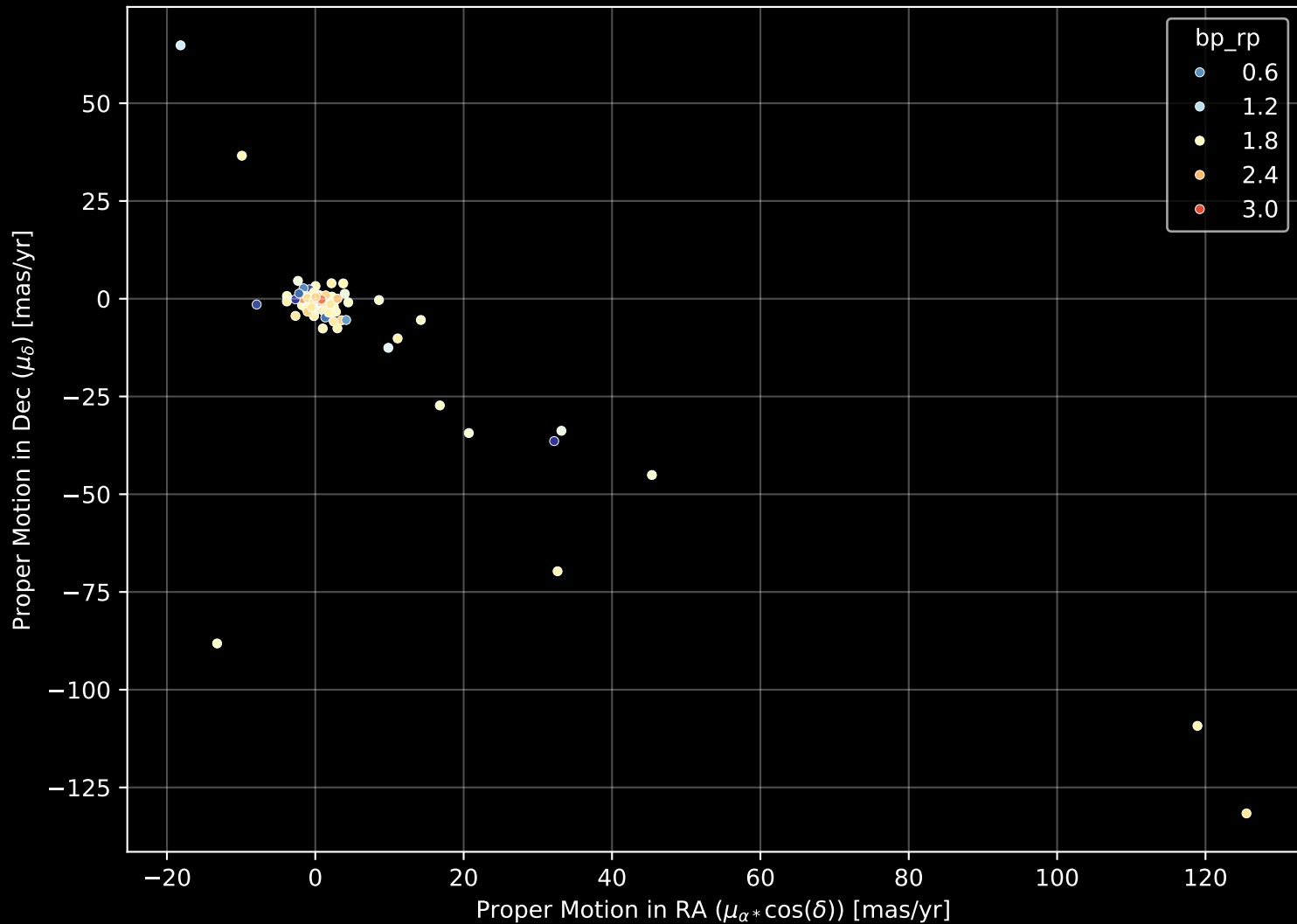
APOGEE DR17 Field: [146+04] Proper Motion Diagram (n= 197)
