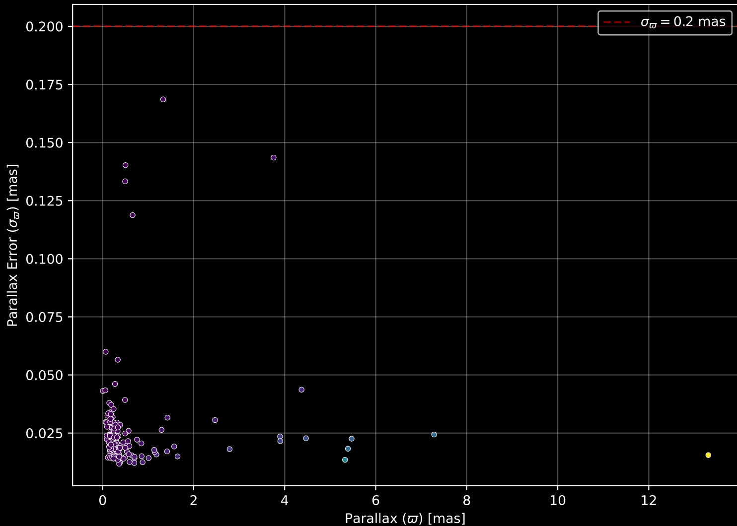
APOGEE DR17 Field: [146+04] Parallax Quality (n= 197)
