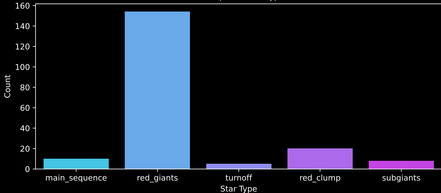
APOGEE DR17 Field: [146+04] Count plot of Star Type
