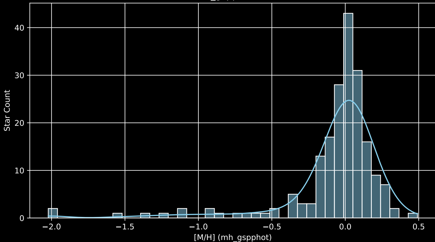
APOGEE DR17 Field: [146+04 [M/H] (mh_gspphot) (n= 194)
