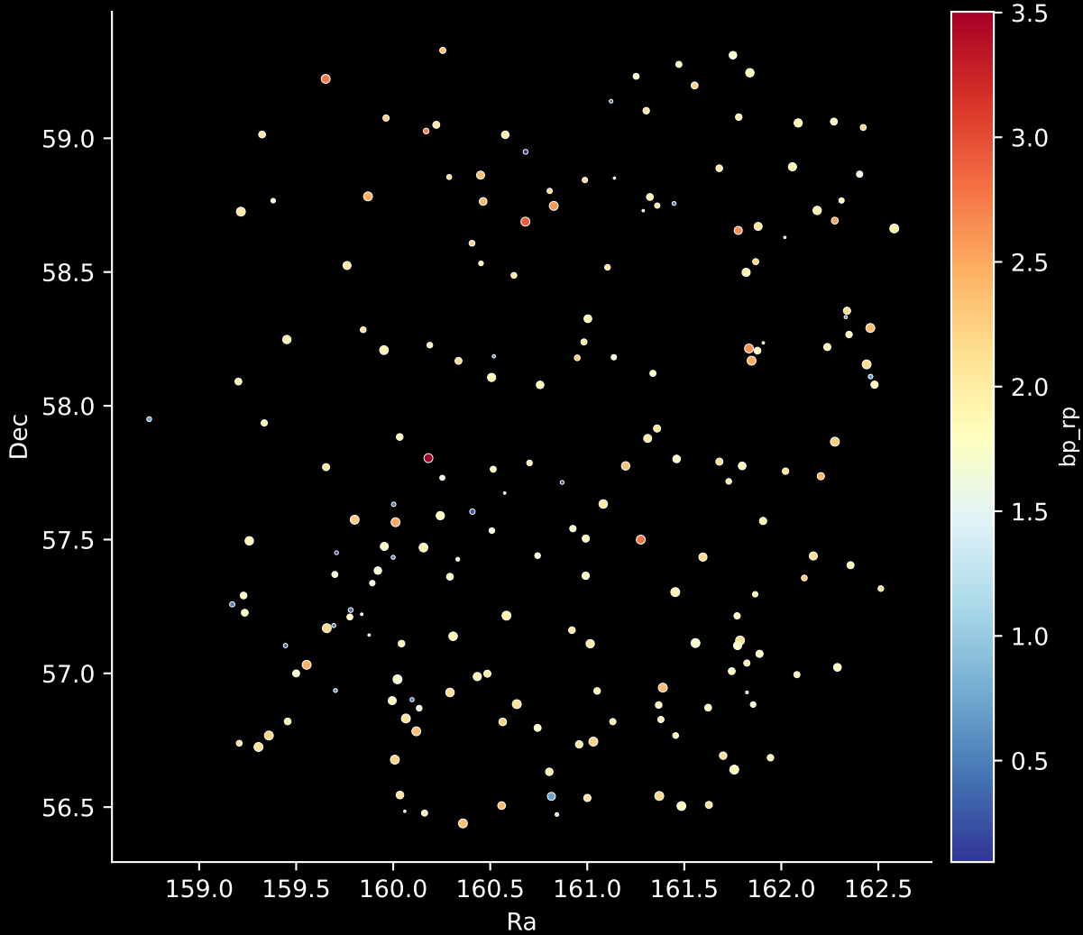
APOGEE DR17 Field: [146+04] Stars: 197
