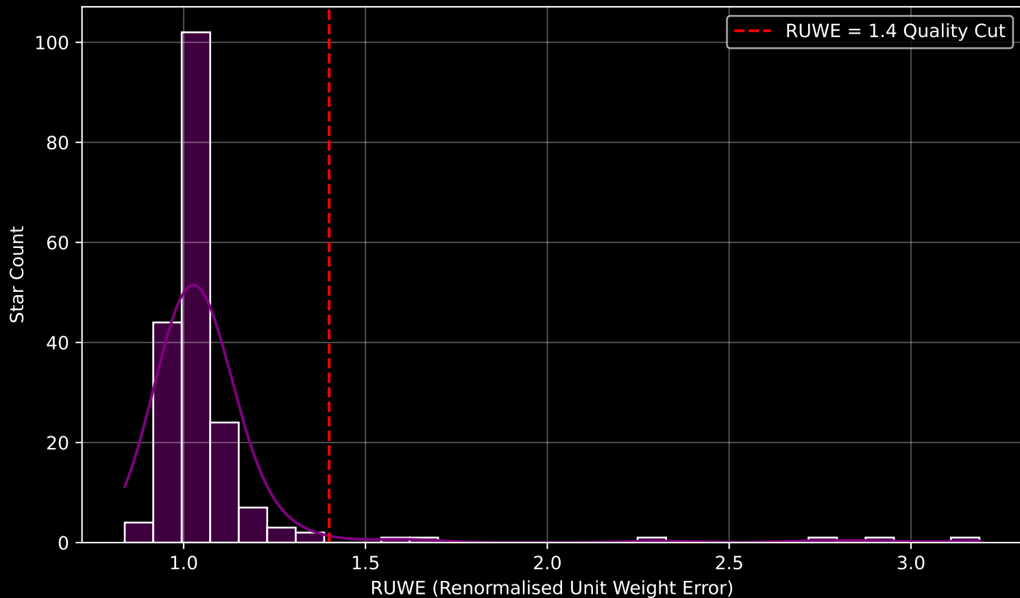
GAPOGEE DR17 Field [146+04] RUWE Distribution (n= 192)
